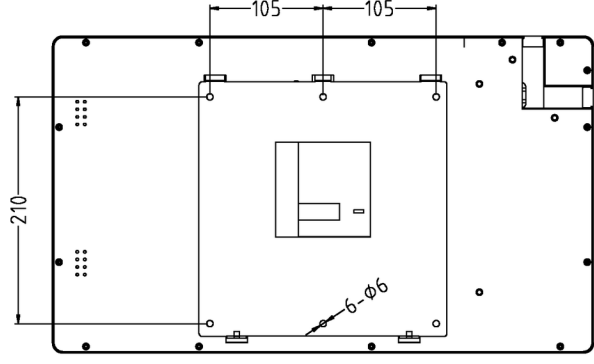
Mounting holes · 210 × 210 mm
