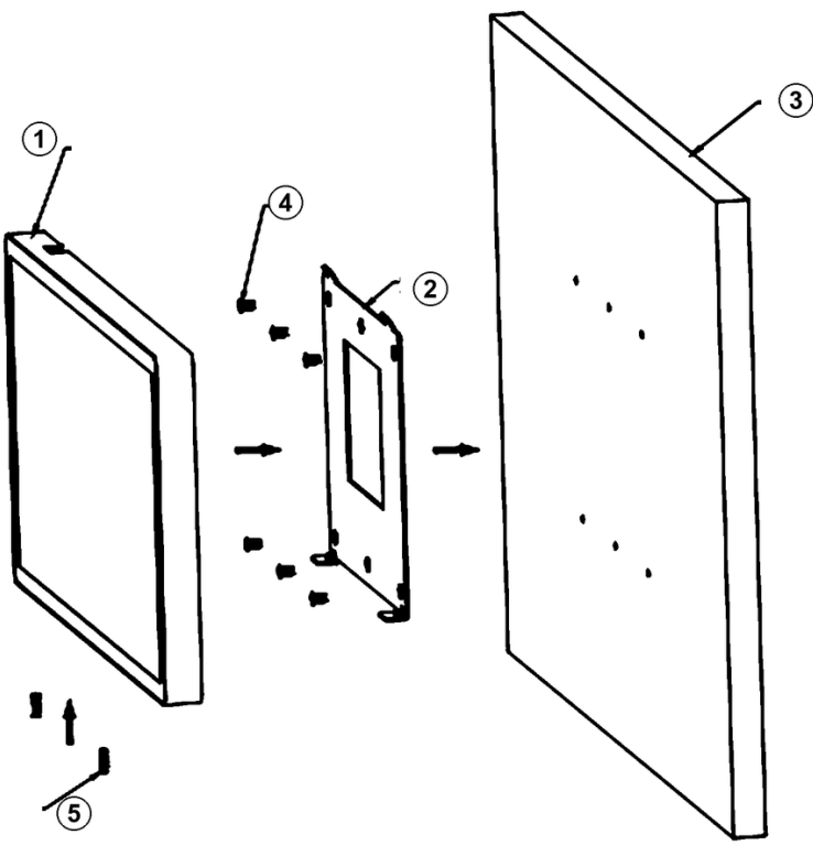
Fig. 1 · Wall-mount assembly (exploded view)
